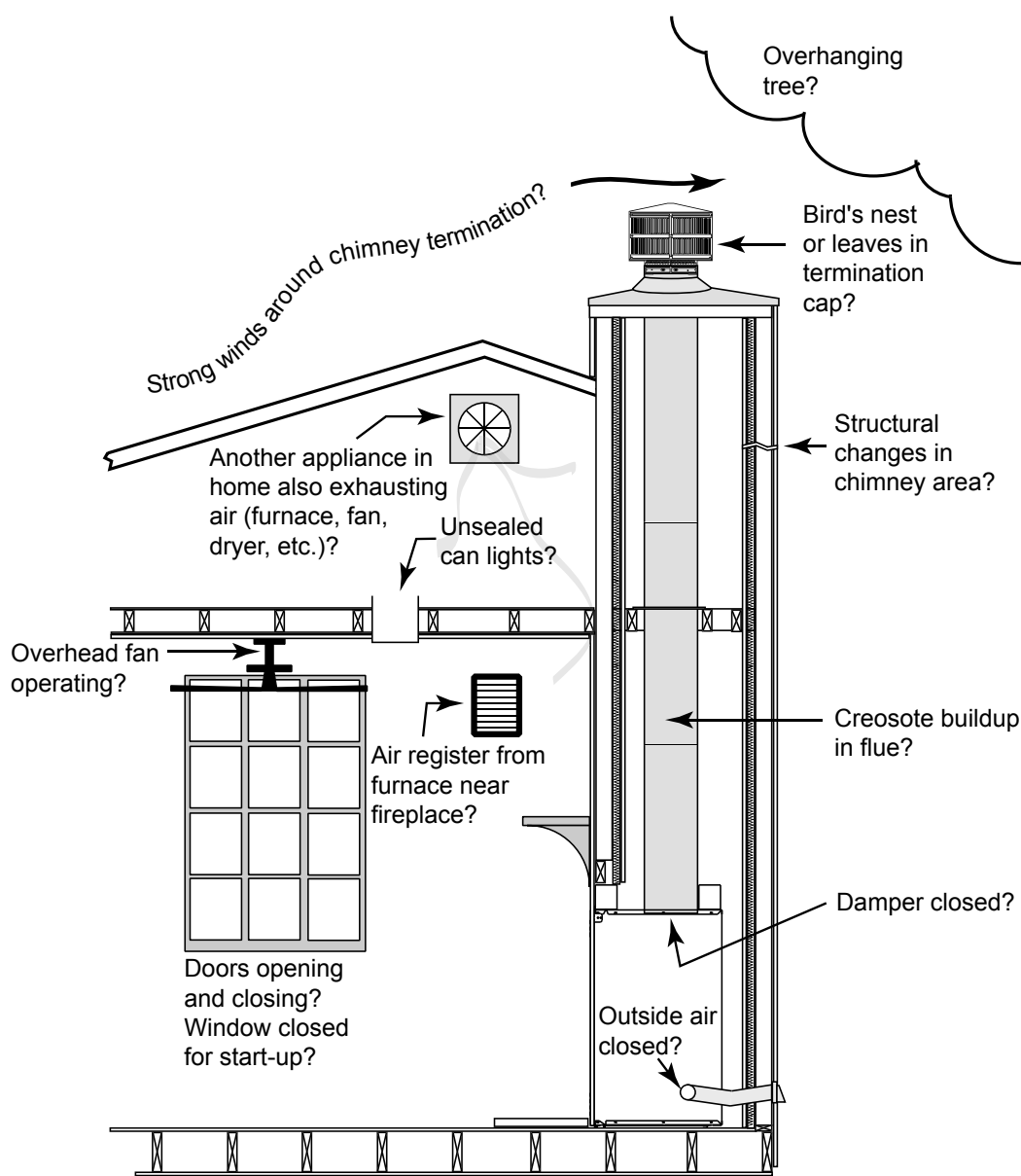
Figure 10.1 Factory-built Fireplaces: Troubleshooting
