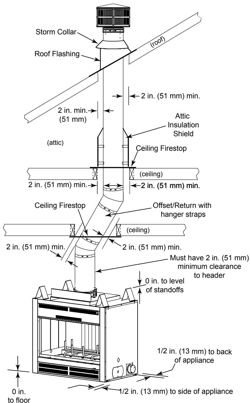
Figure 3.2 Clearances to Combustible Materials
