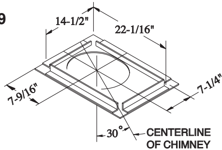
SF30 FIRESTOP SPACER
