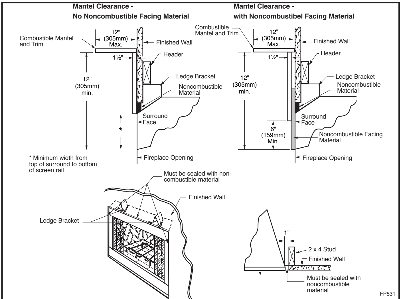
Fig. 22 Mantel clearance.
