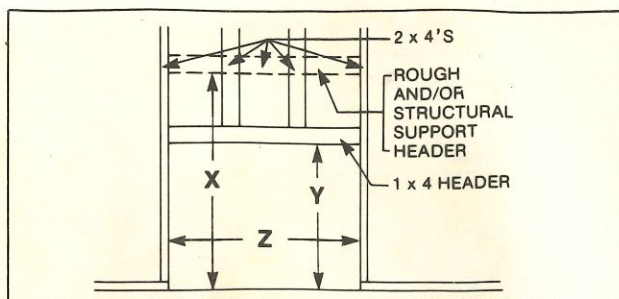
Fig. 15. Dimensions of fireplace opening.
