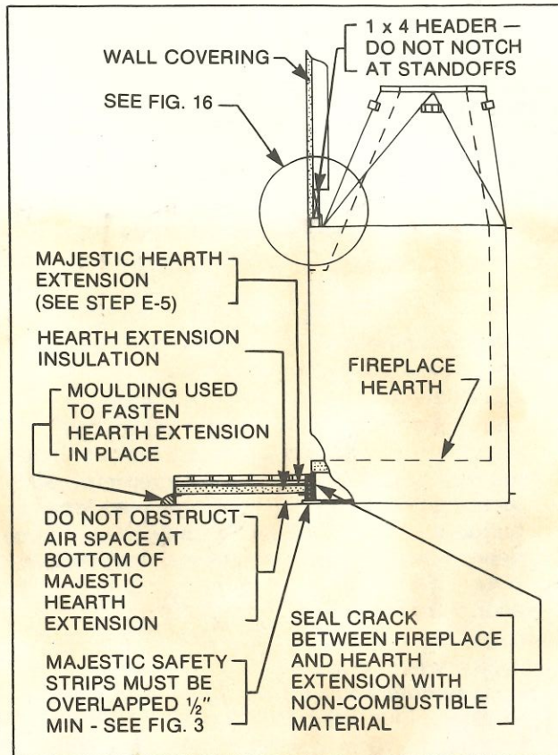
Fig. 18. Sealing detail.
