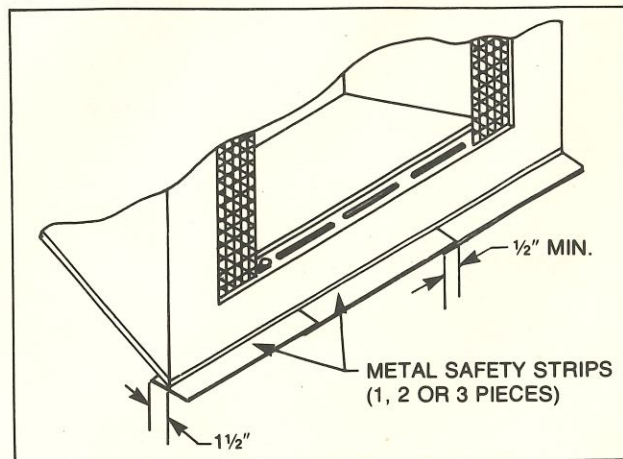
Fig. 3. Install metal strip(s) under front of fireplace.
