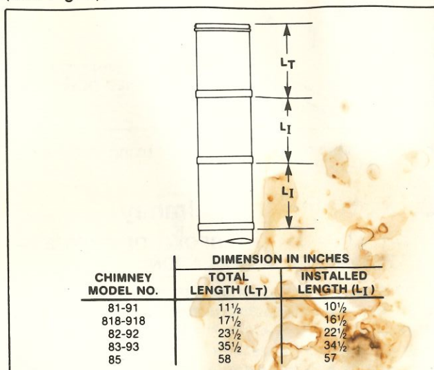
Fig. 2. Installed lengths of chimney sections.
