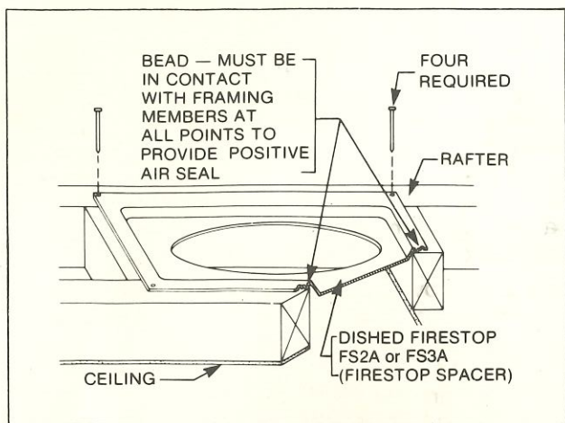
Fig. 11. Position of firestop when area above ceiling is an attic.
