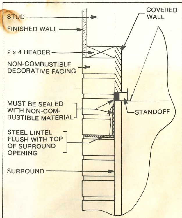
Fig. 17. Facing on fireplace surround flush with finished wall.
