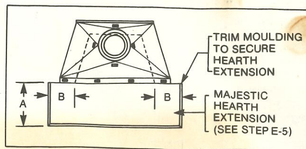
Fig. 21. Minimum dimensions of the hearth extensions.
