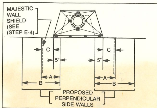
Fig. 20. Protect adjacent combustible side walls with Wall Shield(s).
