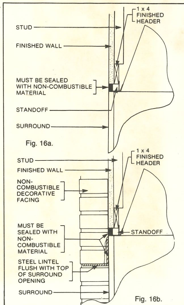
Fig. 16. Fireplace surround flush with finished wall.
