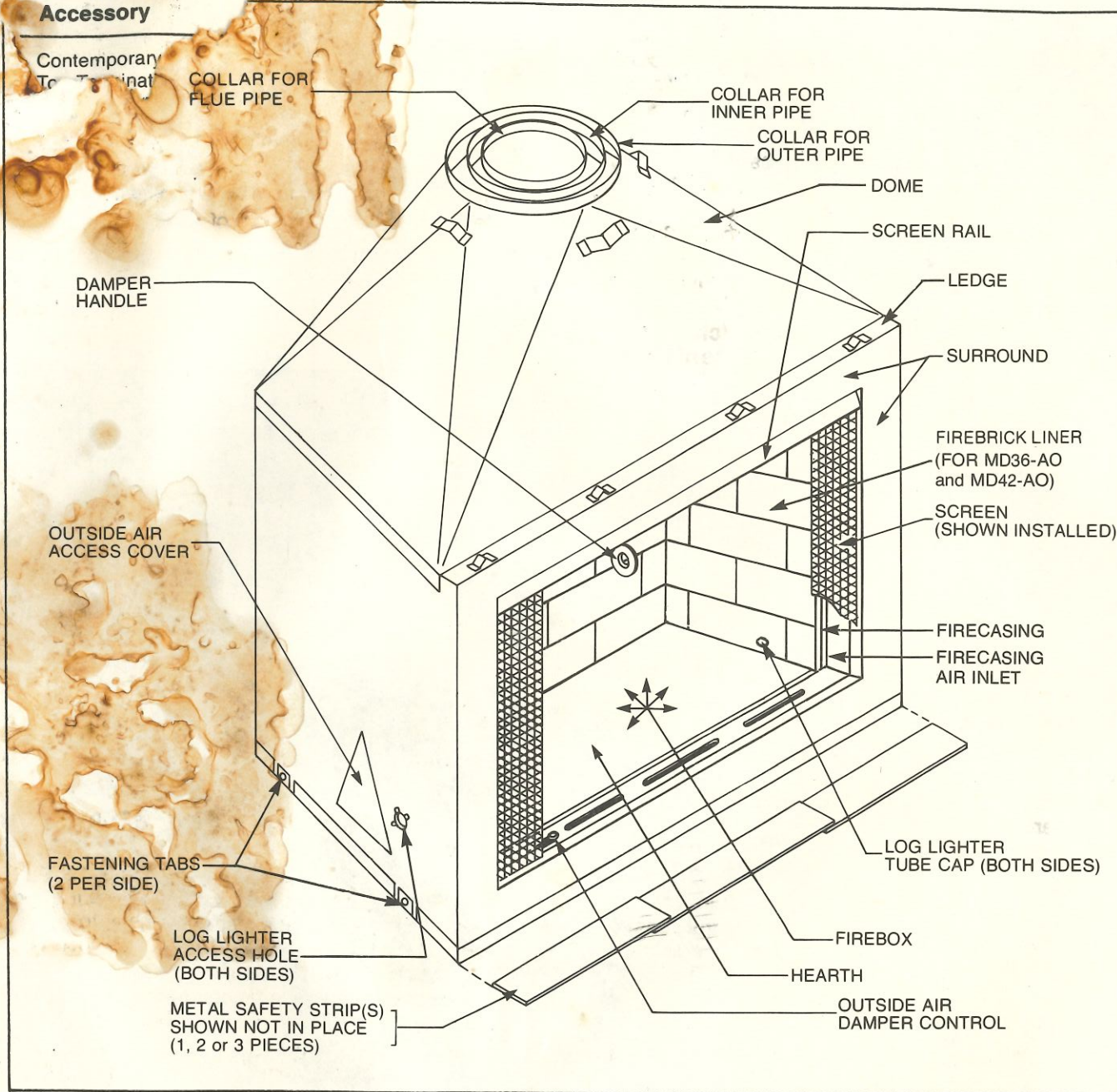
Fig. 1. Parts of the MAJESTIC M28-AO, M36-AO and MD36-AO and MD42-AO fireplaces.
