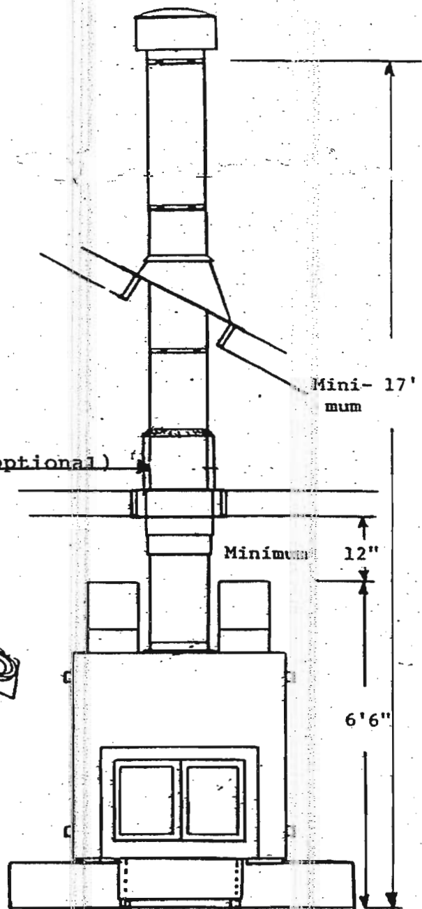
ADJUSTABLE FLASHING
