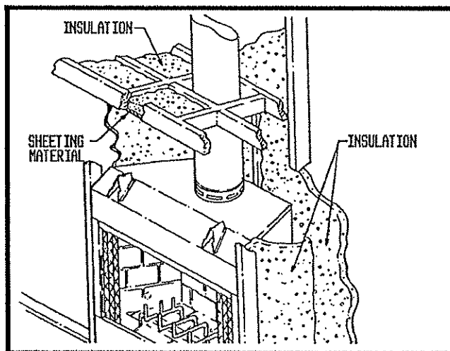
Fig. 16. Additional insulating methods.
