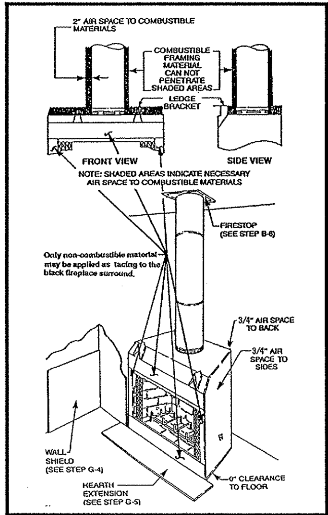
Fig. 27. Minimum air spaces to combustible materials.
