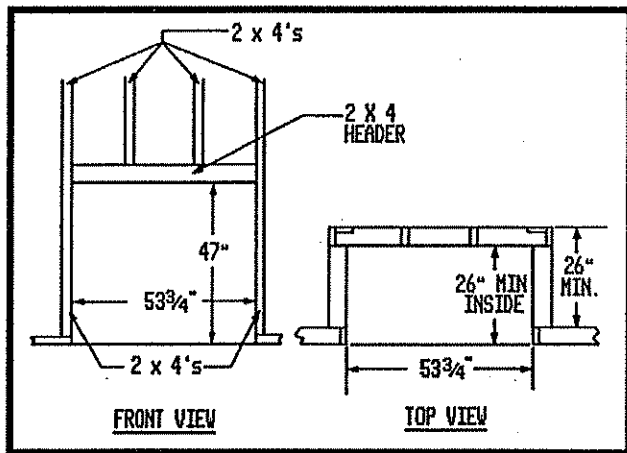
Fig. 17. Minimum fireplace enclosure dimensions.
