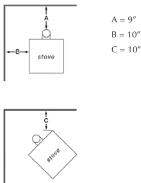
Clearances to combustibile Materials
