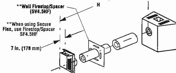
Figure 36 - Rear Vent - NO ELBOWS - Square Horizontal Termination (SV4.5HTS)
