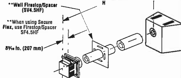
Figure 37 - Rear Vent - NO ELBOWS - for D-500 and DR-500 models only - Small Square Horizontal Termination (SV4.5HTSS)
