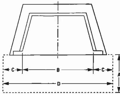
Hearth Extension Dimensions
