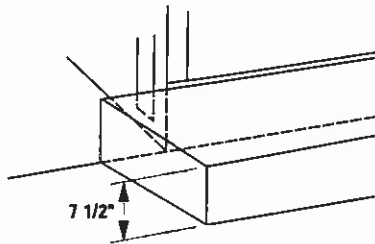
Max. Thickness Of Hearth Extension When Non-Circulating Models Are On The Floor
