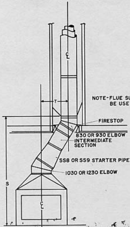
USING 30° ELBOWS & SS8 or SS9 STARTER PIPE
