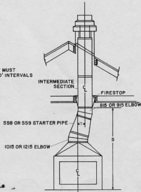
USING 15° ELBOWS & SS8 or SS9 STARTER PIPE
