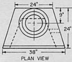
PLAN VIEW
